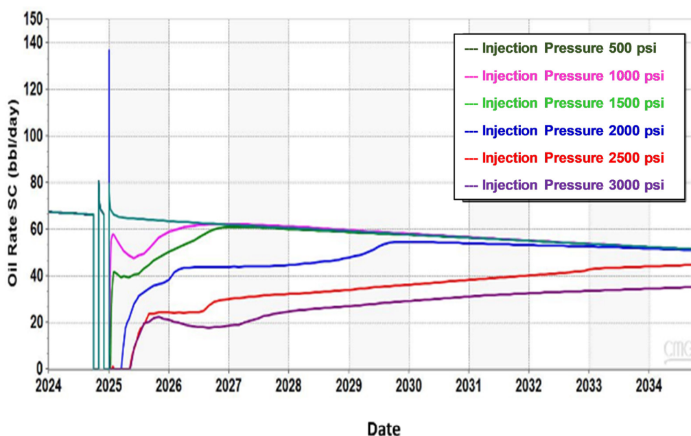
Figure 9. Oil rate at various injection pressure
