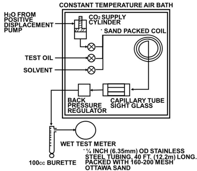
Figure 1: Schematic of slimtube apparatus (After Stalkup1983) [1].
