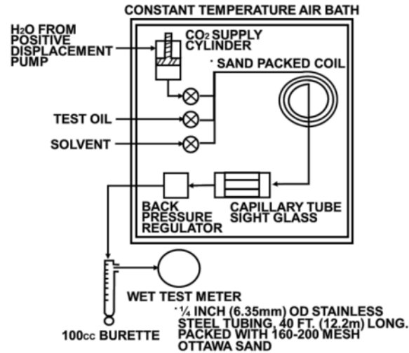
Figure 1: Schematic of slimtube apparatus (After Stalkup1983) [1].
