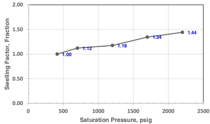
Figure 5: Correlation results of swelling factor to saturation pressure.
