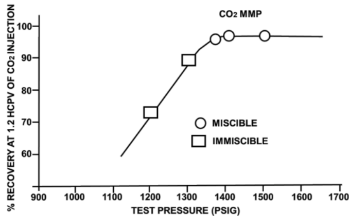
Figure 2: MMP determination on CO 2 -Oil displacement (After Stalkup 1983) [1].
