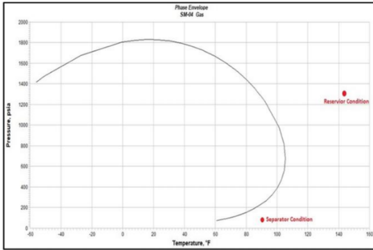
FIGURE 5. Fluid Phase Diagram of SM-04 Well
