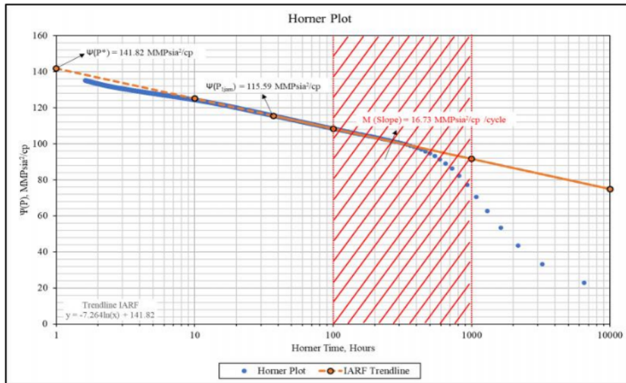
FIGURE 7. Horner Plot Graph of SM-04 Well
