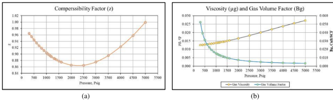
FIGURE 4. Compressibility Factor Curve (a), Gas Viscosity and Gas Volume Factor Curve (b)
