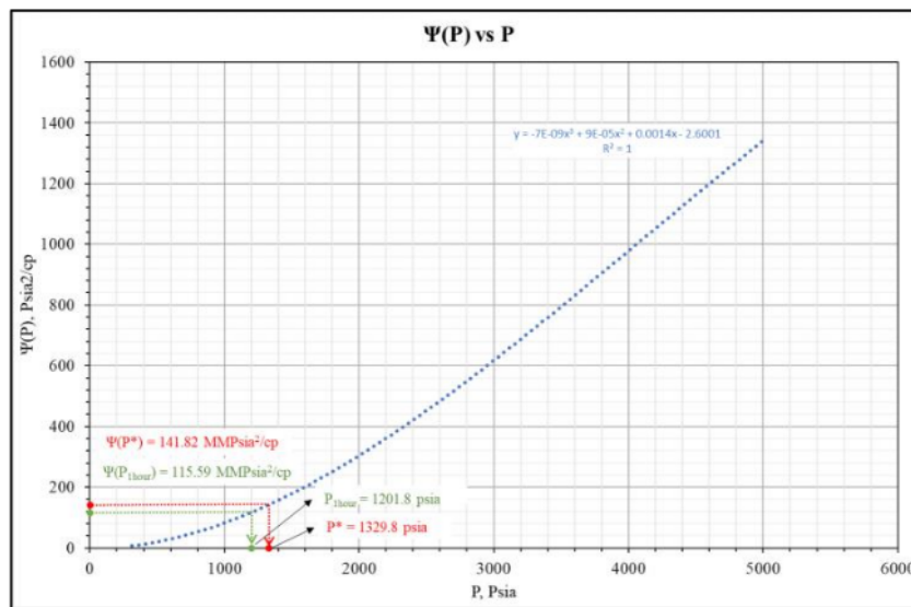
FIGURE 8. Pseudo Pressure ( \Psi ) Conversion Graph
