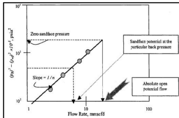
FIGURE 2. Deliverability Curve [3]
