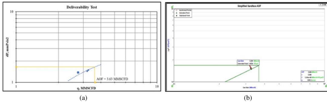
FIGURE 10. Deliverability Curve of SM-04 Well by Rawlins-Schellhardt Equation (a) and IHS Well-test Software (b)
