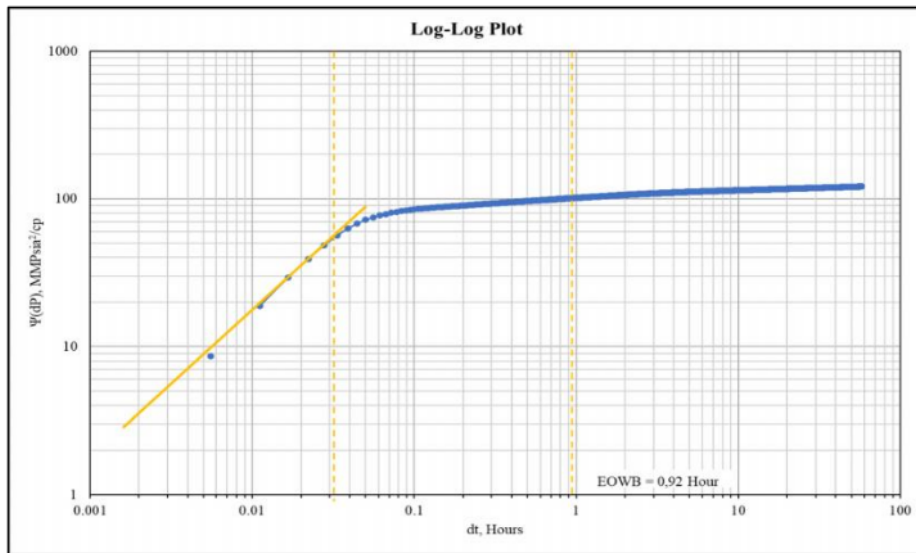
FIGURE 6. Log-Log Plot Graph of SM-04 Well
