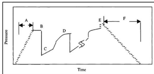
FIGURE 1. Pressure Record in Drill Stem Test (DST) [4]
