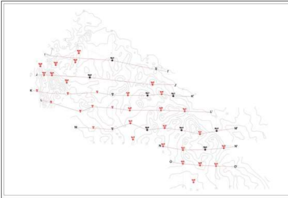
Gambar 15. Peta sayatan penampang bor ( drill ) di area extension PT. Holcim Indonesia (Tbk)
