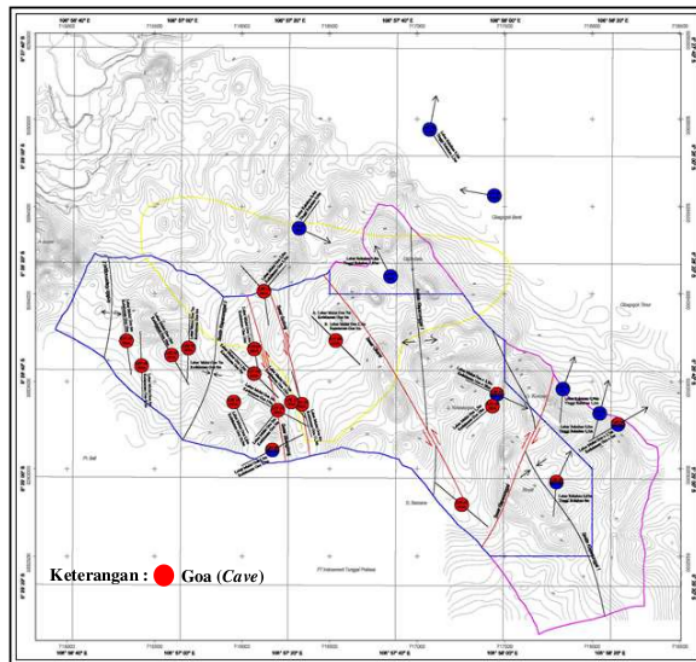
Gambar 6. Peta persebaran goa (cave) di area extension
