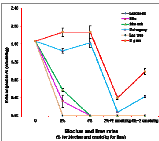
Figure 7. Soil exchangeable Al as affected by biochar and lime amendments
