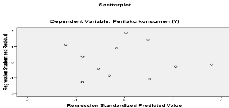
Fig 1. Linearity test Regression Line
