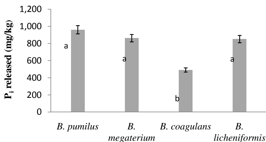
Fig. 6. The P_i released from cassava leaf meal using different bacterial phytase sources after 1 h incubation at pH 6.0 at 37 °C (300 \mu l enzyme + 600 \mu l substrate + 900 \mu l 5% TCA). Bars represent means \pm S.D. Means with different letters are significantly different ( P < 0.05 )
