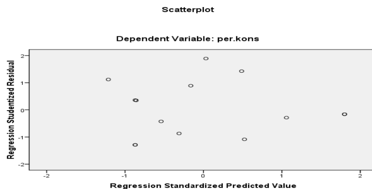
Fig 2. Heteroscedasticity Test
