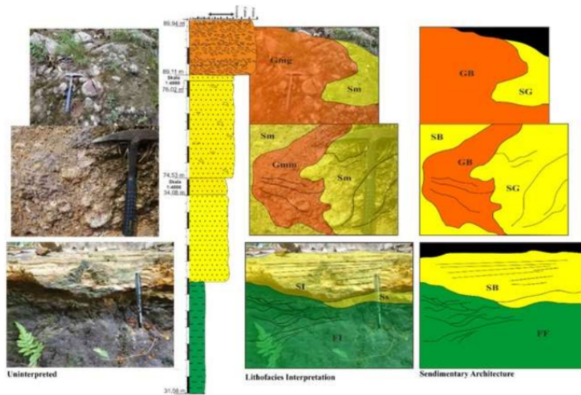
Figure 5. Interpretation of architectural elements in sandstone-conglomerate deposits
