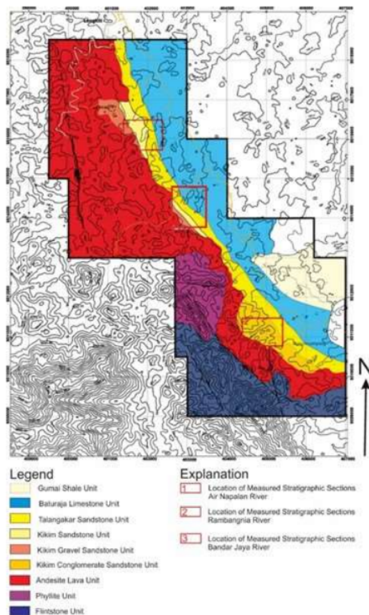
Figure 1. Geological map of Bungincampung village research area, Simpang District, South Ogan Komerung Ulu Regency, South Sumatra Province
