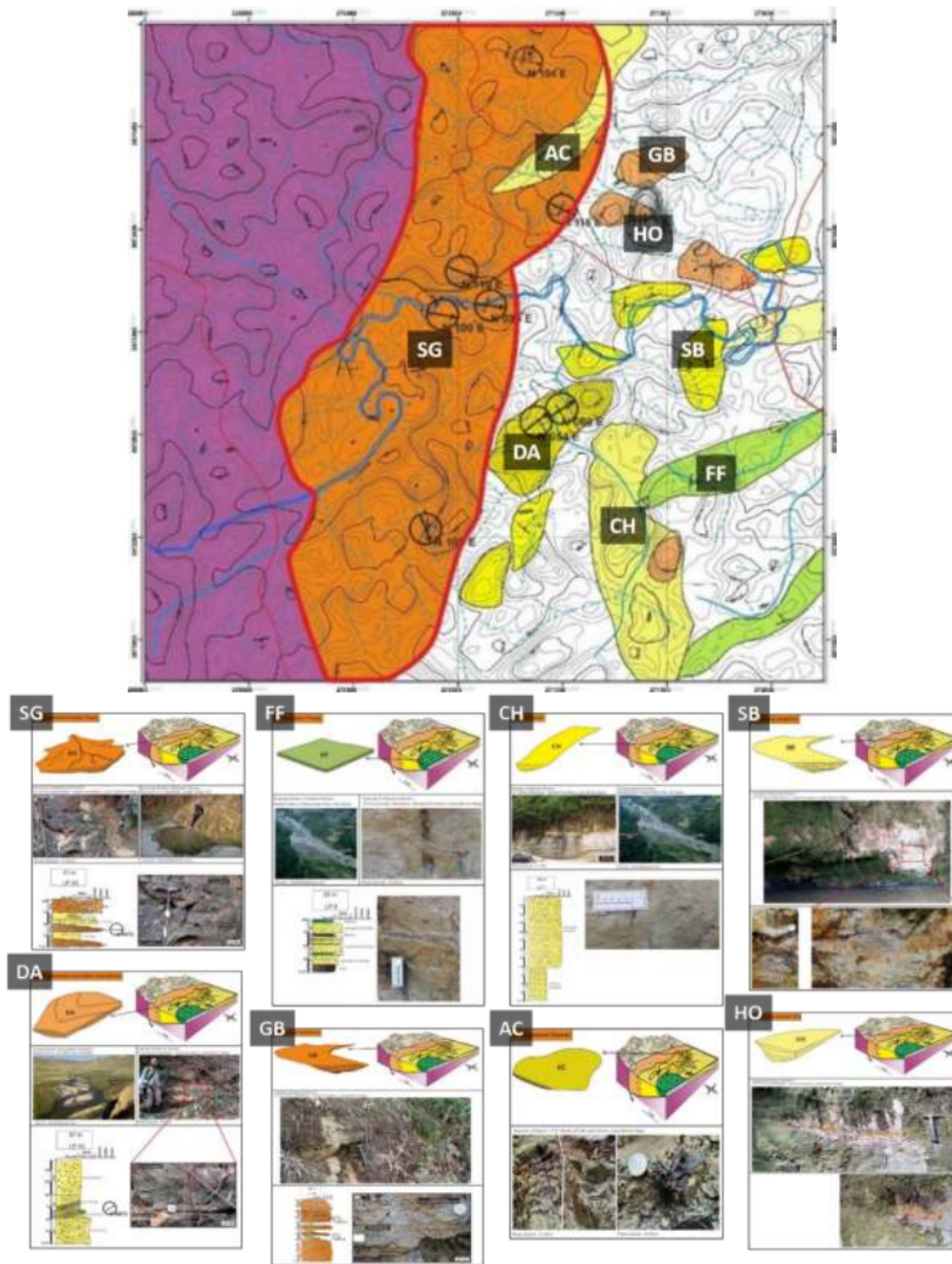
Figure 8. The Architectural elements of the investigation area.
