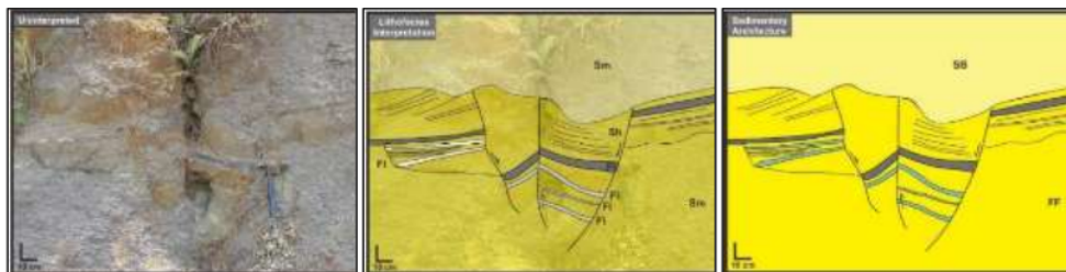
Figure 7. Architectural element Benakat tuffaceous-sandstone unit
