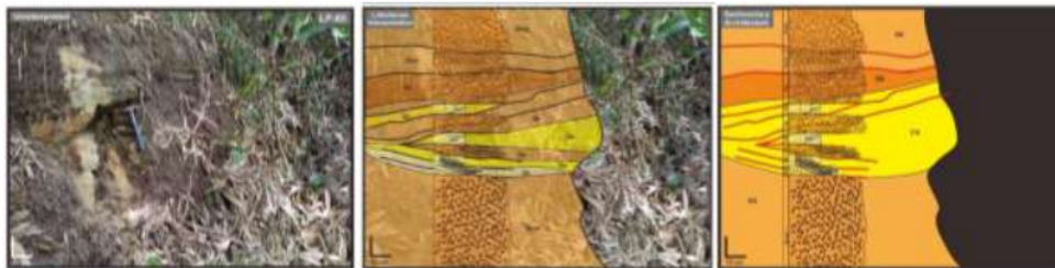
Figure 5. Architectural element of depositional Lemat gravel-sandstone unit
