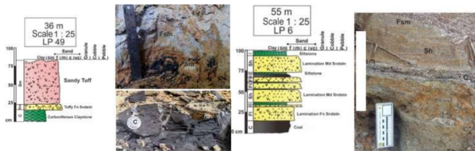
Figure 6. Lithofacies in the Benakat tuffaceous-siltstone
