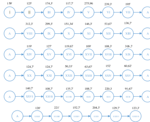
Figure 2. Precedence diagram optimal
