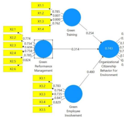
Gambar 2. Outer Model
