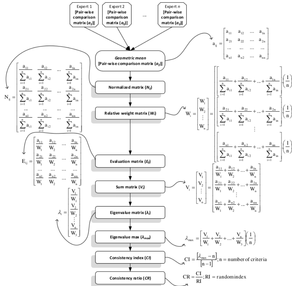
Gambar 3. Alur proses AHP
