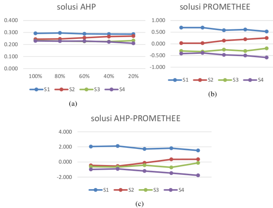
Gambar 4. Analisis sensitifitas (a) AHP, (b) PROMETHEE, (c) kombinasi AHP-PROMETHEE
