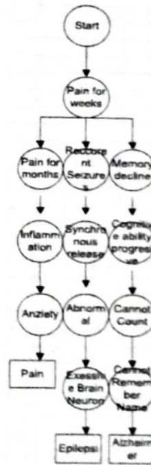
Figure 4. Forward Chaining.
