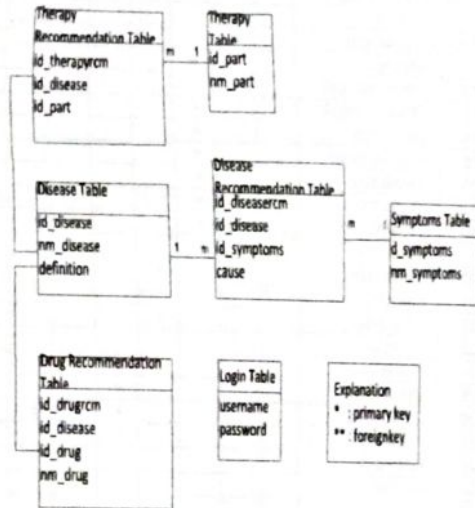
Figure 3. Relationship Table
