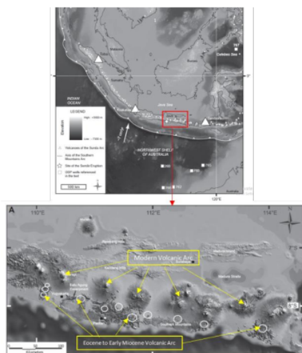
Figure 1. Modern Volcanic arc and Southern Mountain Volcanic Arc (Smyth et.al, 2011)
