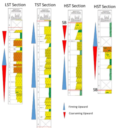
Figure 3. Stratigraphic Section of Tebing Breksi from bottom to top (from left to right)
