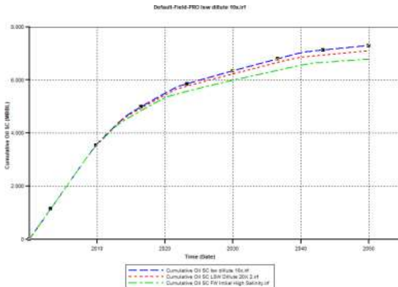
Gambar 3.5. Cumulative Production
