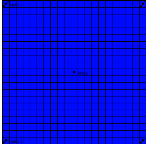
Gambar 3.1. Model Reservoir 2D
