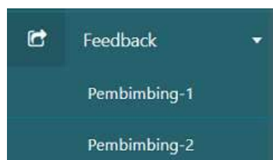
Gambar 3.10 Menu Feedback
