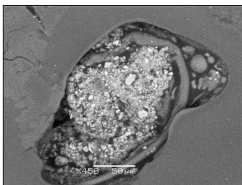
Fig 8. Photomicrography of SEM shows pyrite minerals that fill inertinite group maceral
