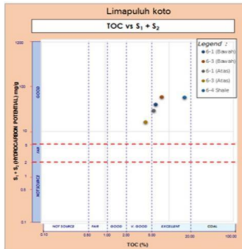
Gambar 10. Plot data antara S1 + S2 Vs TOC
