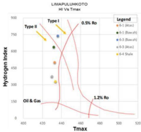
Gambar 13. Plot data HI Vs Tmax
