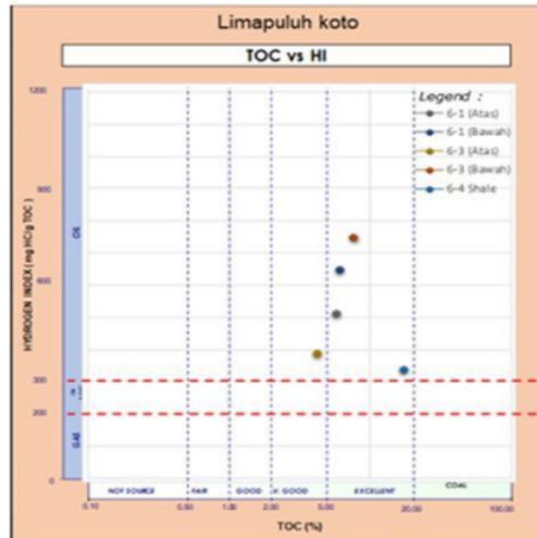
Gambar 11. Plot data HI Vs TOC
