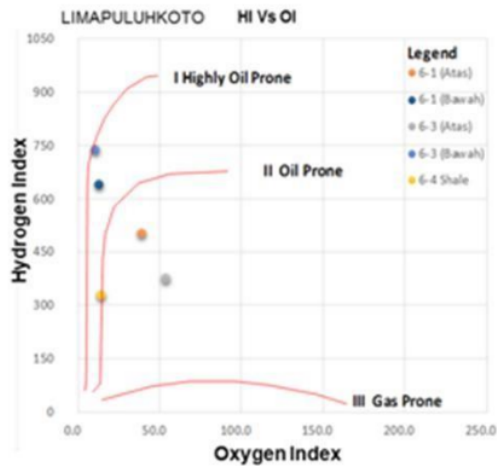
Gambar 12. Plot data HI Vs OI
