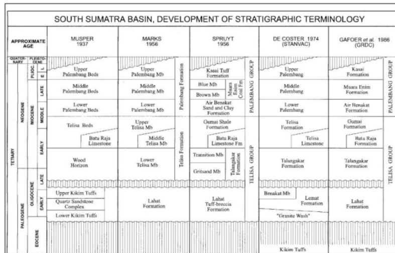
Fig 2. Regional Stratigraphy (de Coster, 1974; Ginger and Fielding 2005).
