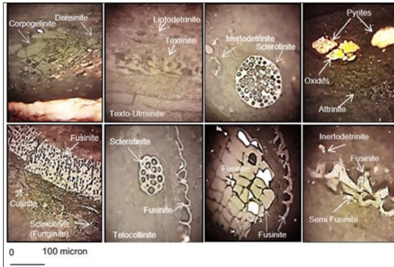
Fig 5. Coal Microscopic of Seam A-1
