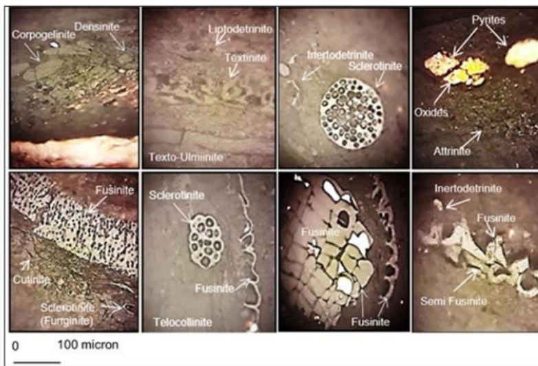
Fig 5. Coal Microscopic of Seam A-1
