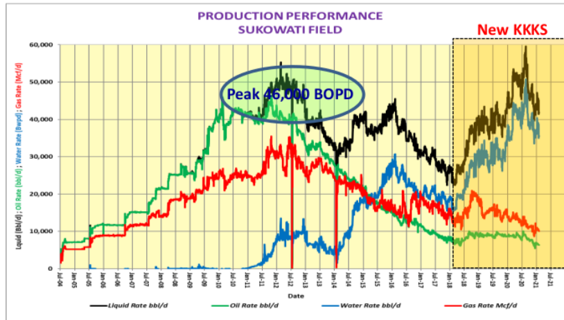
Image 1.HAS Field Production Performance
