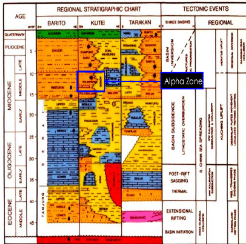
Figure 3. Regional stratigraphy of Kutei basin [6].
