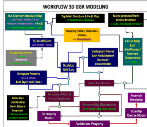
Figure 4. Workflow of 3D modeling of SKK Migas [7], [8].
