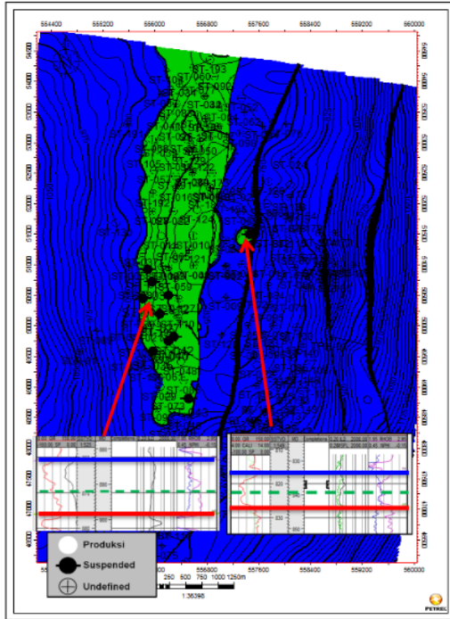
Figure 10. Fluid contact map of Alpha zone.
