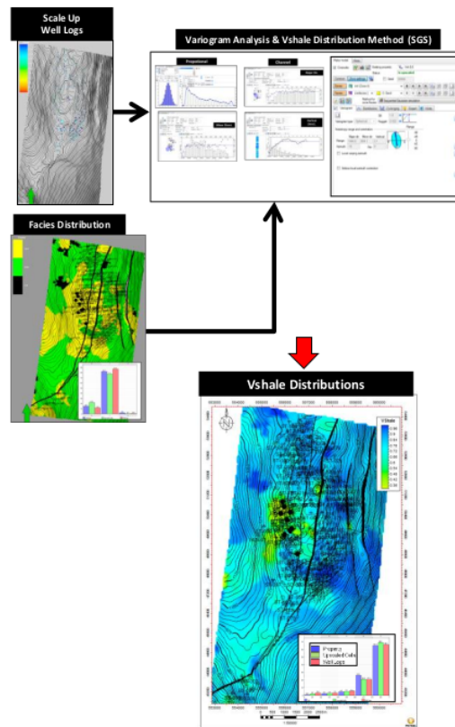
Figure 13. 3D Property modeling process.
