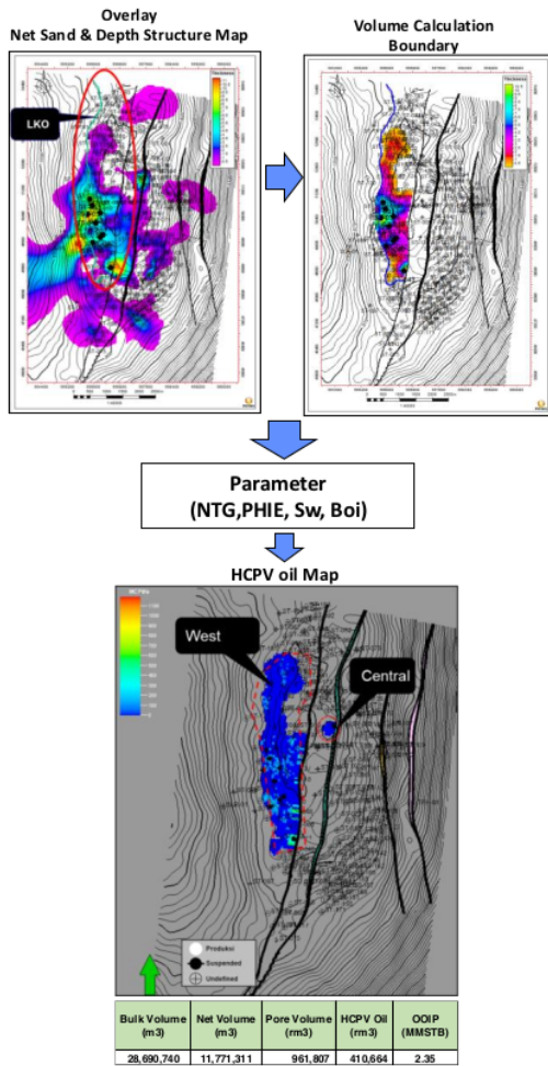
Figure 15. Alpha zone OOIP determination result.
