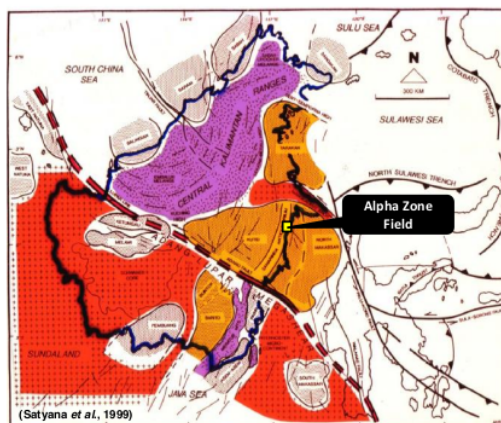
Figure 1. Location of observation study [6].
