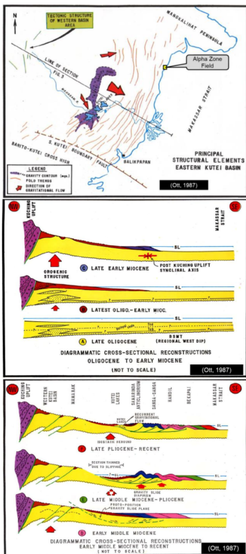
Figure 2. Kutei basin development [2], [5], [6].
