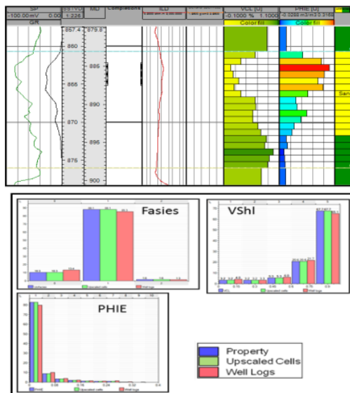
Figure 9. Layering and scale-up of well logs.
