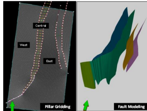
Figure 5. Pillar gridding and fault modeling.
