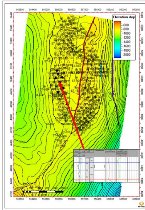
Figure 8. Alpha zone depth structure map.
