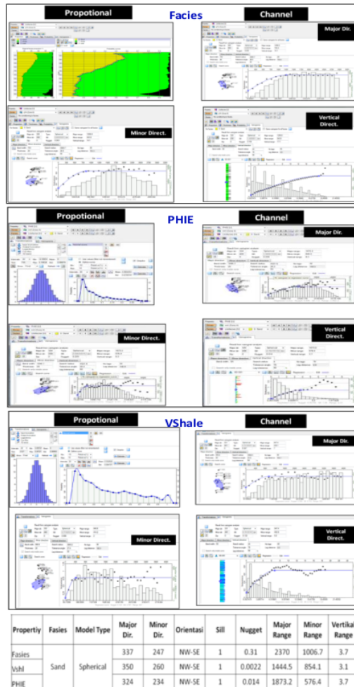
Figure 11. Variogram geostatistical analysis.
