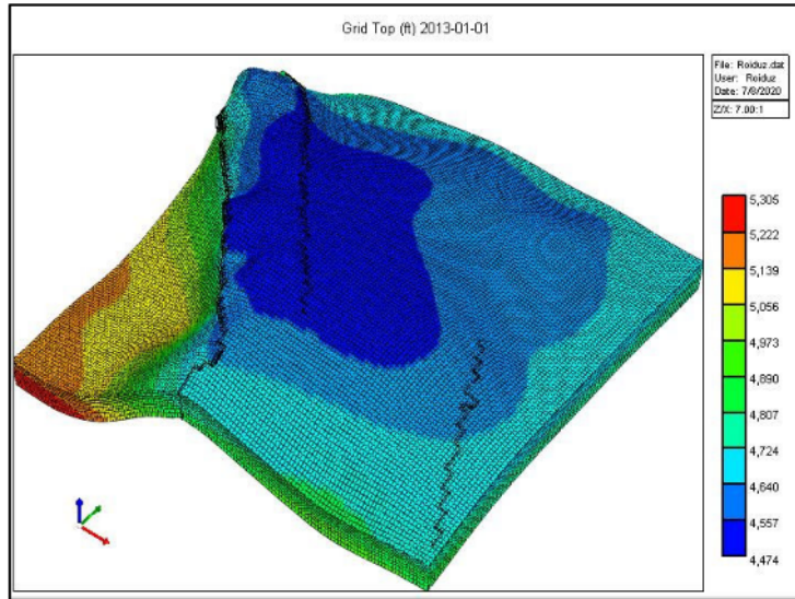
FIGURE 1. Grid Top of RZ Field Reservoir
