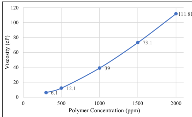
FIGURE 2. Viscosity vs Concentration of FP360S Polymer
