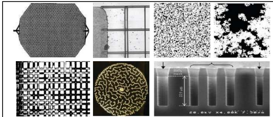
Figure 1. Micromodels Made by Previous Researchers [8, 13-17]
