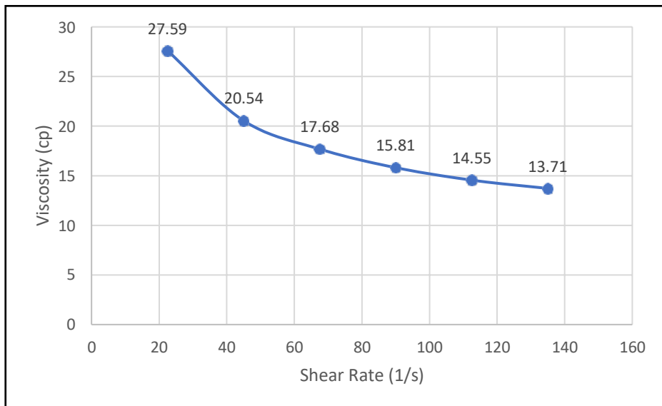
Figure 8. Polymer Solution Viscosity vs Shear Rate (2000 ppm)
