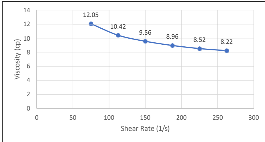
Figure 7. Polymer Solution Viscosity vs Shear Rate (1500 ppm)
