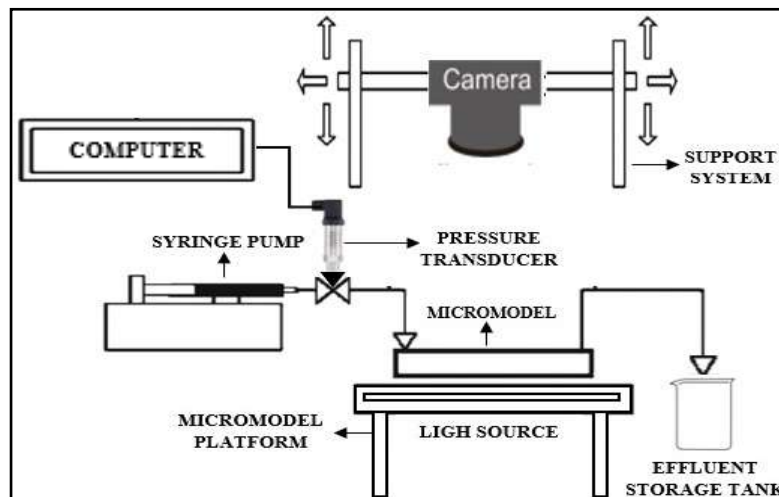
Figure 3. Micromodel Flooding Step
