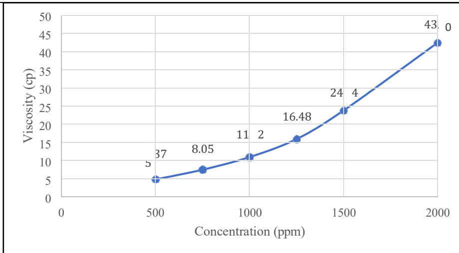
Figure 5. Polymer Solution Viscosity vs Concentration
