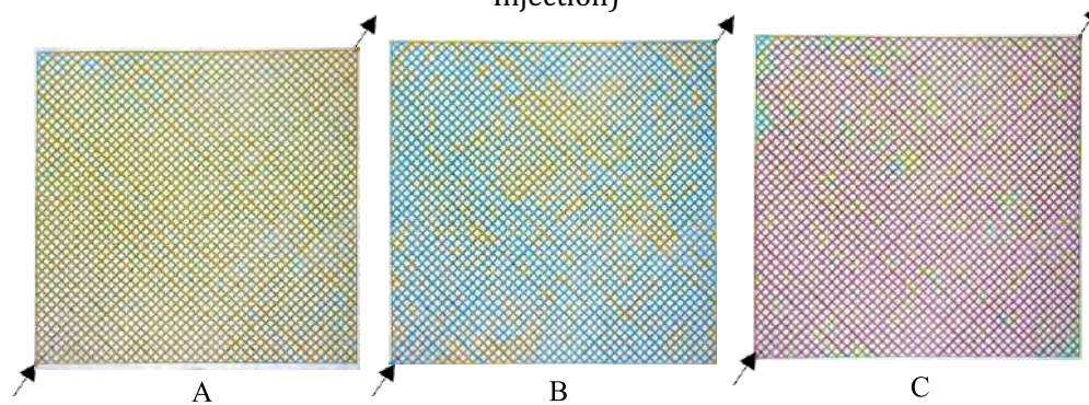
Figure 13. Visualization of Micromodel Flooding Test for Scenario 3 (A = Initial Condition, B = Waterflooding, C = 2000 ppm Polymer)
