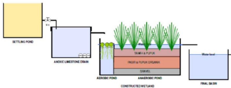
Gambar 1. Skematik sistem passive treatment
