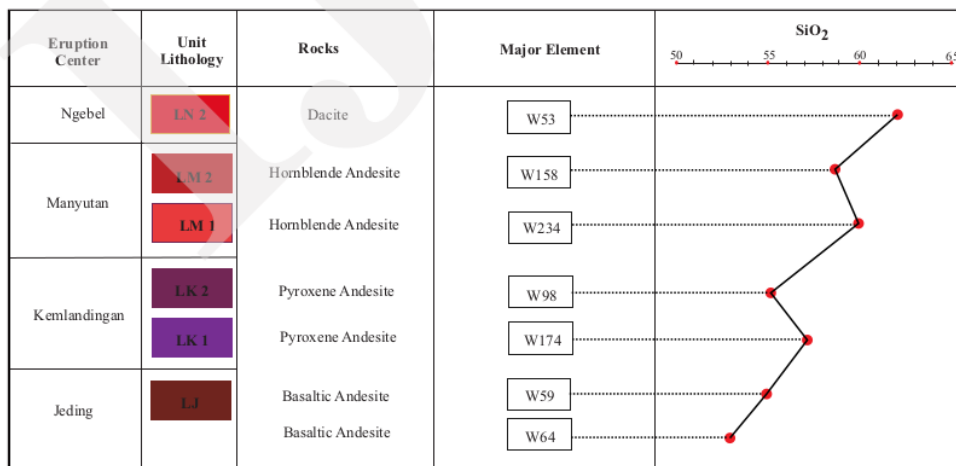
Figure 7. Evolution of magmatism of the NVC.
