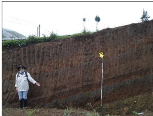
Fig 17. Outcrop of pyroclastic fall lapilli-tuff in the pyroclastic fall Merdada 2 unit was abundant and interspersed with several pyroclastic fall deposits.
