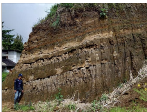
Fig 11. The pyroclastic outcrop fell lapilli-tuff in the Dieng Kulon unit, which was abundant and interspersed with several pyroclastic fall deposits.
