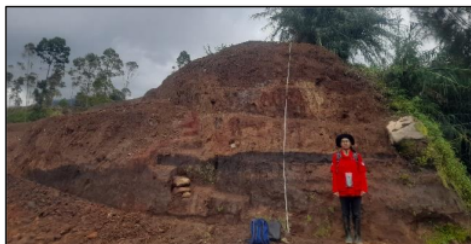
Fig 4. The outcrop showing the pyroclastic flow Gembol deposit unit has a massive structure with andesite fragments and contains pumice.
