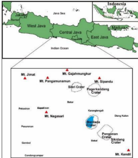
Fig 1. Research area map of Dieng Volcano
