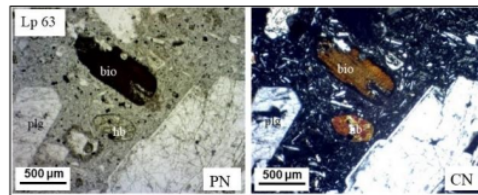
Fig 21. Petrographic of hornblende-biotite andesite shows the presence of plagioclase, pyroxene, hornblende, biotite and opa minerals. At the edges of biotite and hornblende it is seen that it was altered by the mineral opaque. These phenocrysts are surrounded by micro plagioclase forming an intergranular texture. plg: plagioclase; bio: biotite; hb: hornblende; opq: opaque mineral; PN: parallel nicol; CN: cross nicol
