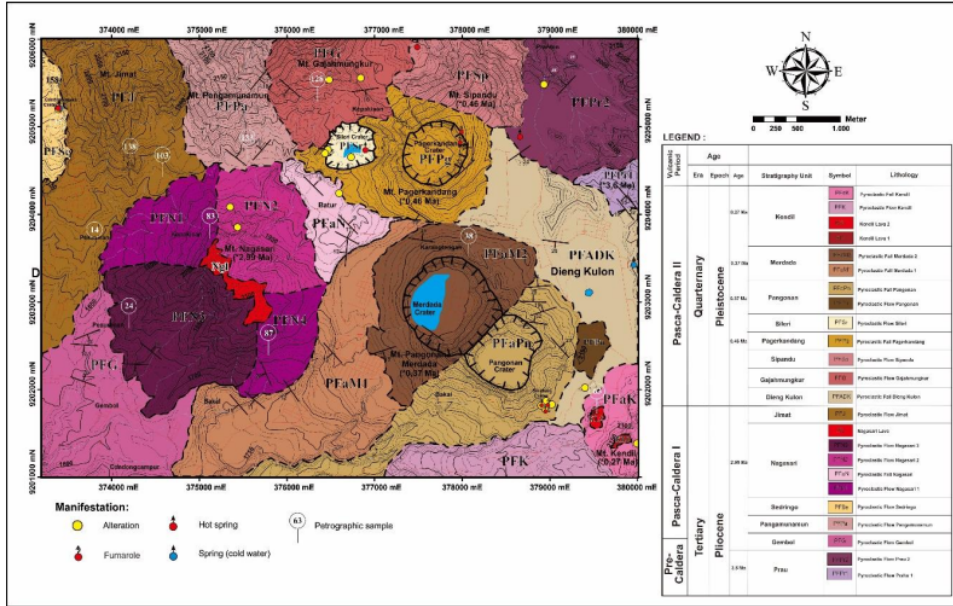
Fig 22. Geological map of the study area.
