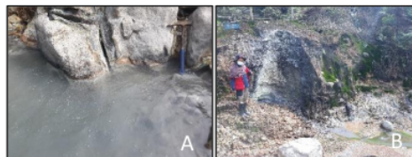
Fig 6. Outcrop of the pyroclastic flows breccia in the pyroclastic flow Sedringo unit (A and B). The breccia fragments consist of pyroxene andesite: plagioclase, pyroxene, opaque minerals, and glass as groundmass.
