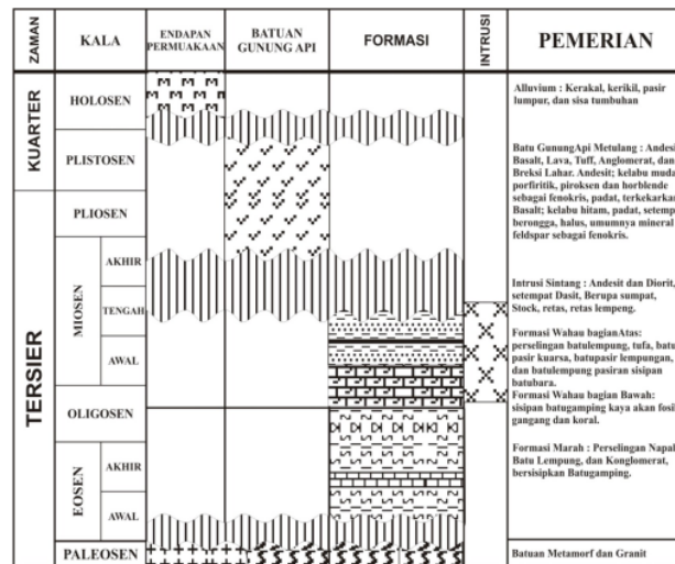
Gambar 3. Stratigrafi Regional Muara Wahau, Kalimantan Timur [8]
