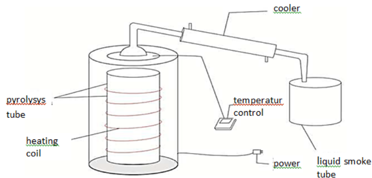
Fig 1. Pyrolysis Apparatus
