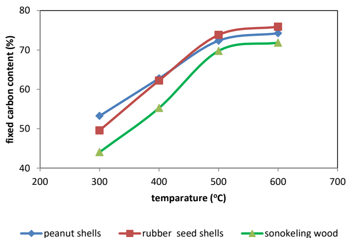
Fig. 5. The effect of temperature on the fixed carbon content
