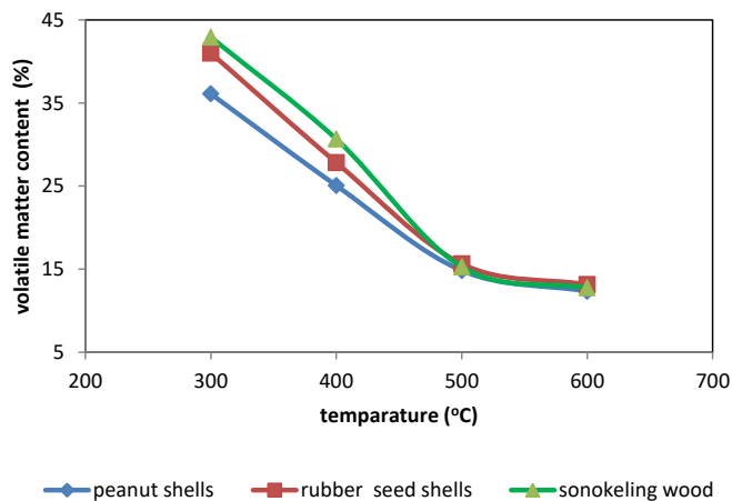
Fig. 4. The effect of temperature on the volatile matter content
