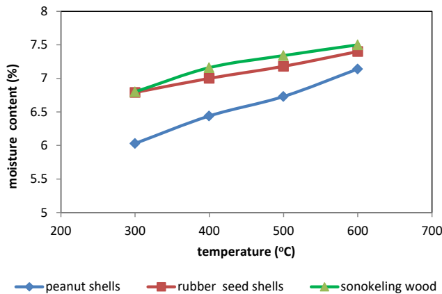
Fig 2. The effect of temperature on moisture content
