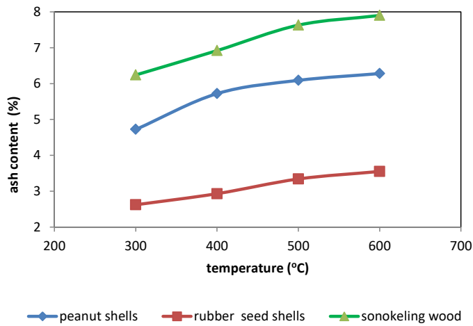
Fig 3. The effect of temperature on ash content
