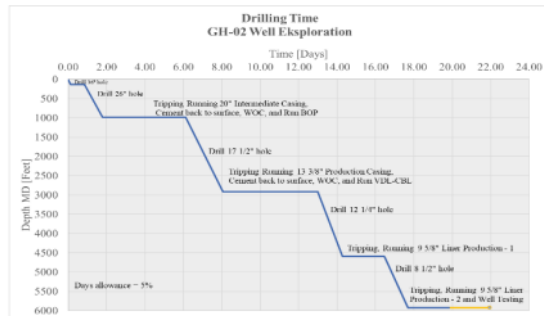
Figure 2 Drilling Time vs Drilling Depth
