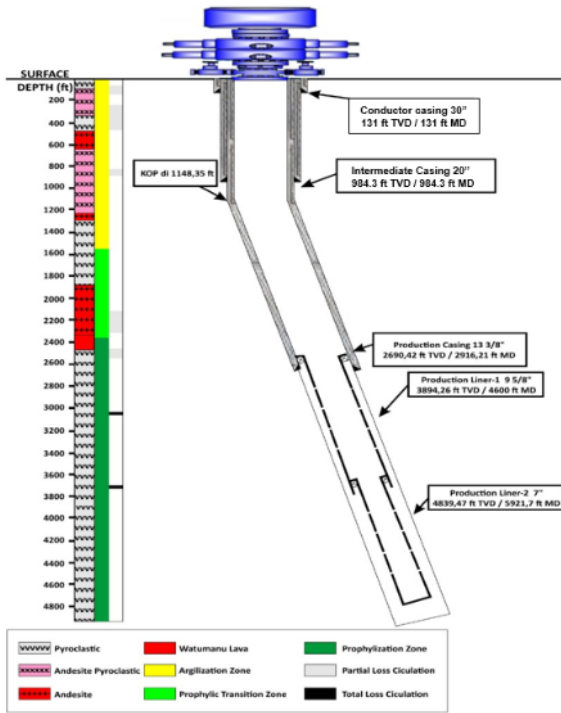
Figure 1 Profile GH-2 Well Exploration
