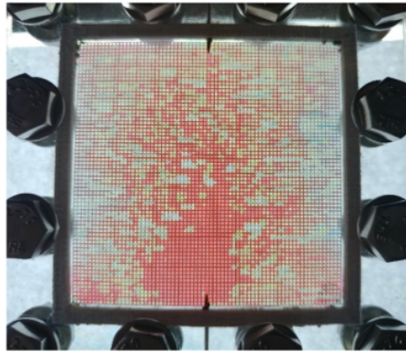
Figure 10. Captured Micromodel Image for 1,000 ppm Polymer Injection
