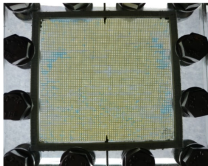
Figure 8. Captured Micromodel Image for Oil Saturation
