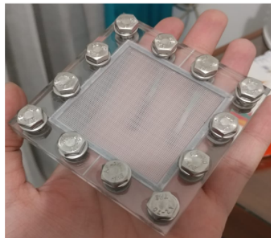
Figure 7. Micromodel Used in Experiment
