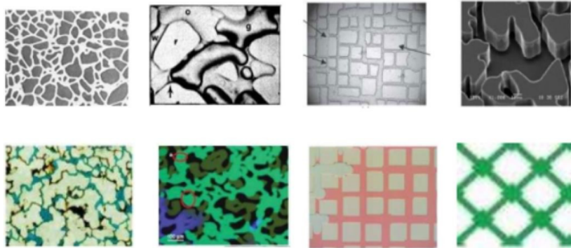
Figure 1. Micromodel Pore Patterns (Source: (Hosseini & Foroozesh, 2019))
