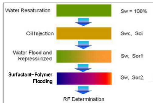
Gambar 2. Mekanisme coreflooding test di laboratorium (After Lemigas, 2012)
