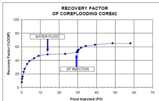
Gambar 8. Hasil coreflooding test-2
