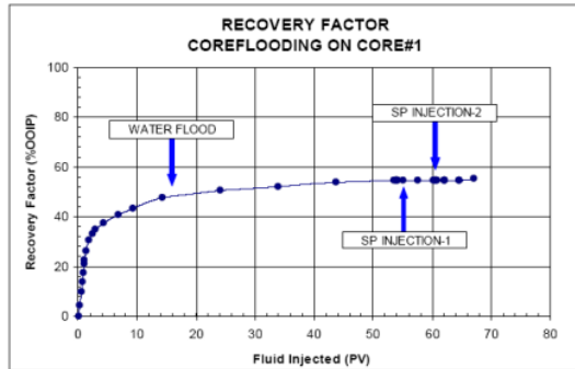
Gambar 7. Hasil coreflooding test-1
