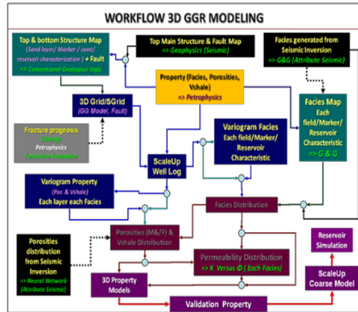
Figure 4. Workflow of 3D modeling of SKK Migas [7], [8].
