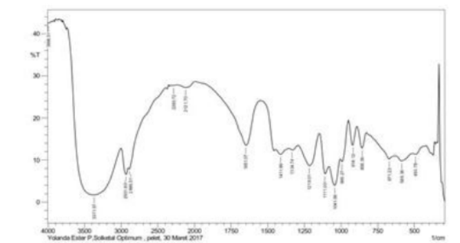
Figure 2. Analysis of the solketal molecular structure using FTIR
