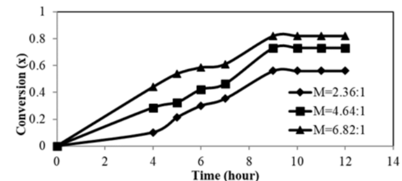
Figure 3 Graph of the relationship between reaction time to Glycerol conversion at different mole ratio of Acetone/Glycerol. The reaction is carried out at a mixed boiling temperature
