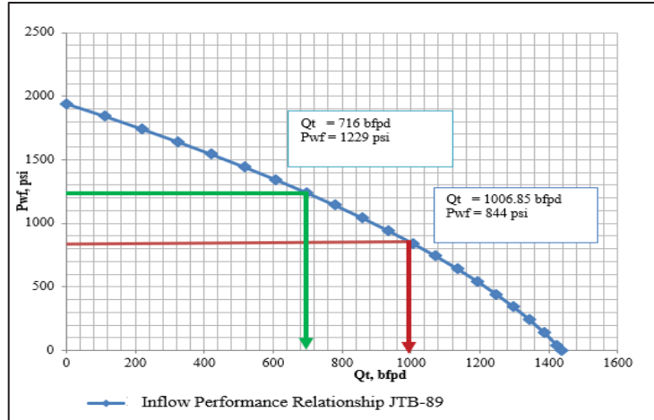
FIGURE 1. Inflow Performance Relationship JTB-89 Well
