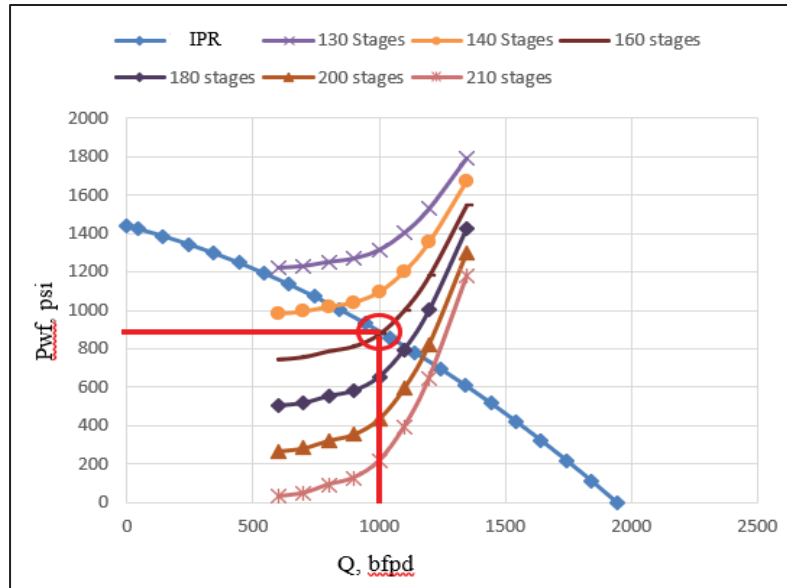
FIGURE 4. Sensitivity of Pump Variable Stages
