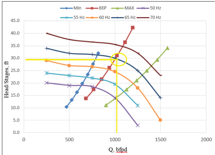
FIGURE 3. Sensitivity of Pump Frequency
