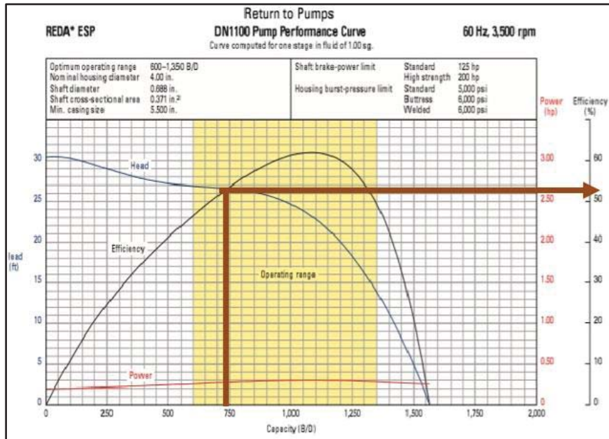
FIGURE 2. Pump Performance Curve of DN1100 Type
