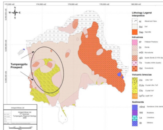
Figure 3. Lithology of the Tumpangpitu prospect area was mapped by PT. Hakman (1999). Hellman (2010)
