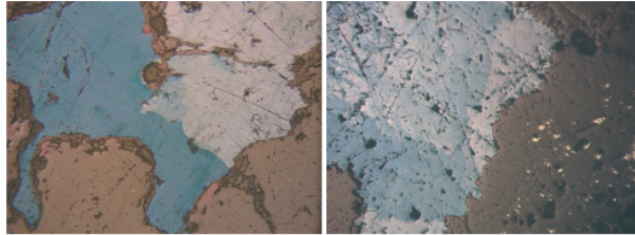
Figure 7. Photomicroscopic of bornite replaced by covellite (left). Pyrite present as inclusions within quartz (gangue) minerals which intergrow with covellite.
