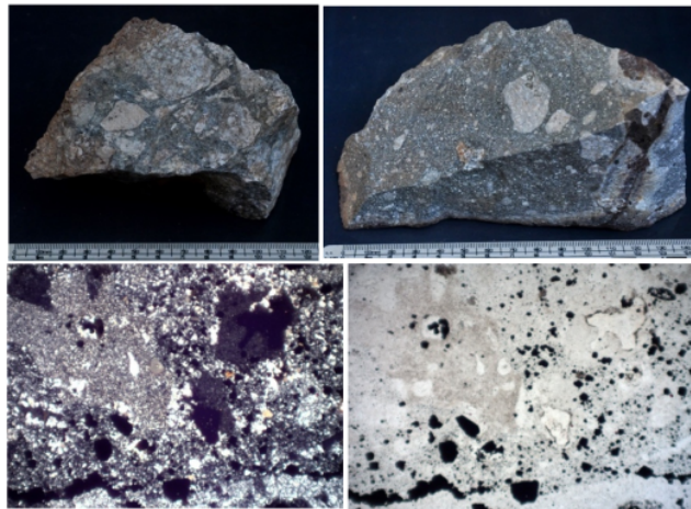
Figure 4 Handspeciment of the phreatomagmatic breccia in pit C (top). Photmicroscopic of the matrix of of the phreatomagmatic breccia.
