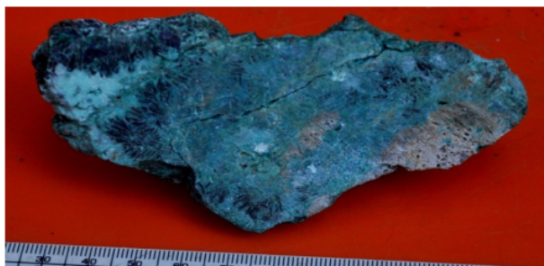
Figure 5. Azurite, mallachiite, and covellite in the phreatomagmatic breccia. Fribrous covellite and malachite infilled within matric the breccia.
