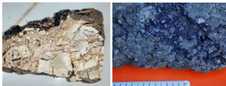
Figure 6 Magmatic hydrothermal breccia that shows Jigsaw Puzzle texture 43 Pit B West (Dynasty Hadyan Saputro and Jalu Bias F) (left). Covellite minerals relaced most of the sulphide minerals and matrix breccia.
