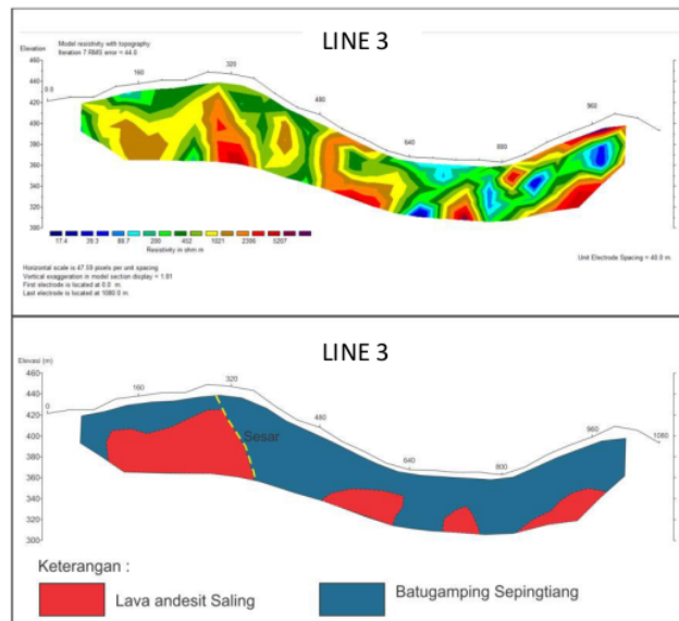
Gambar 6. Penampang Dipole – Dipole Line 3
