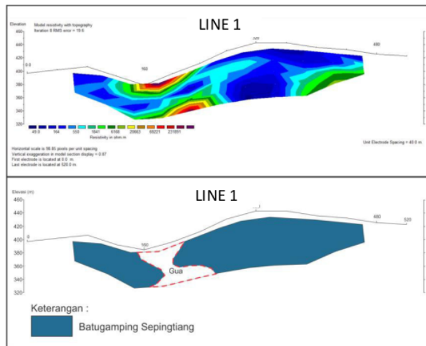
Gambar 4. Penampang dipole - dipole line 1
