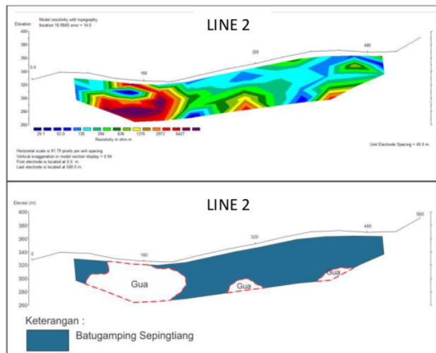
Gambar 5. Penampang dipole - dipole line 2
