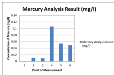
Fig.4 Graph of Mercury Content on Benthic Macroinvertebrate on the Plampang River
