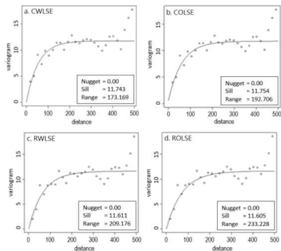
FIGURE 1. The graph of exponential semivariogram base
