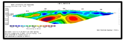
Gambar 4.8. Penampang Resistivitas Lintasan 5
