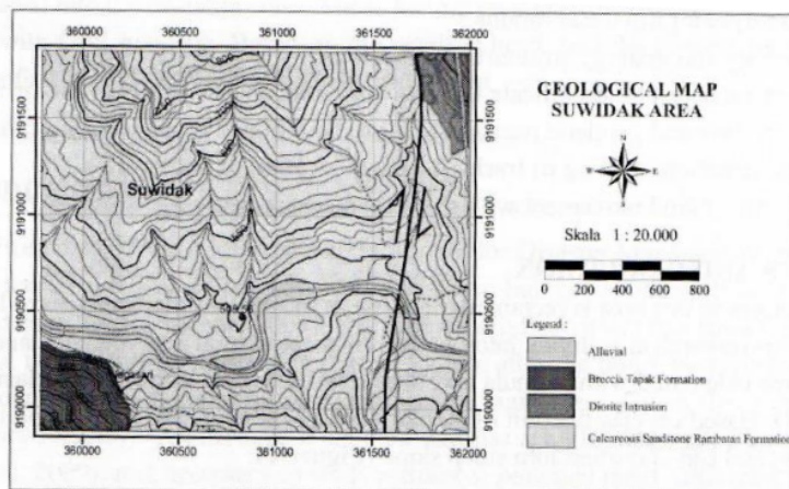
Figure 3. Geological Map
