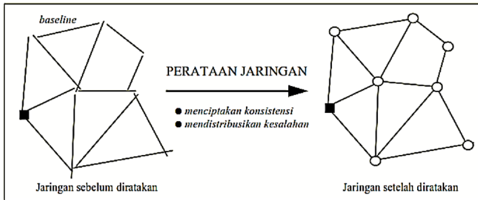
Gambar 17. Perataan jaring GNSS (SNI JKH, 2002)
