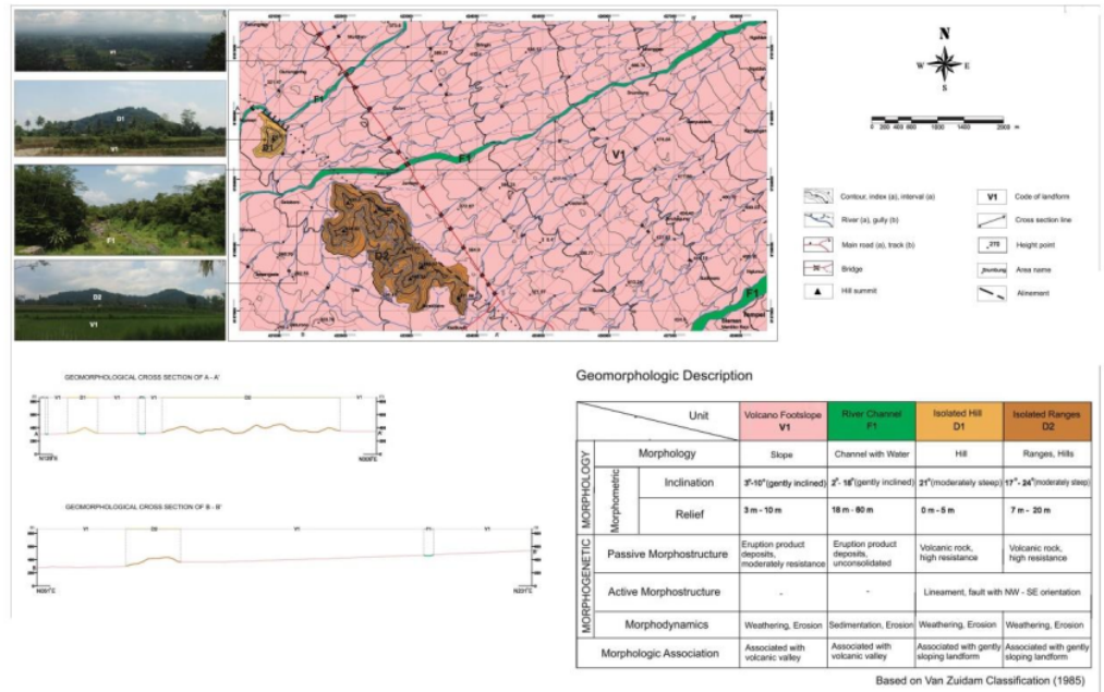
Fig 3. Geomorphological Map of the Research area
