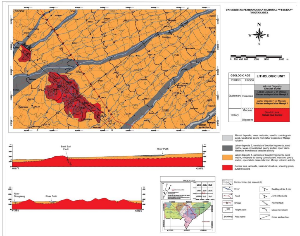
Fig 4. Gerological map of Kali Putih and surrounding area
