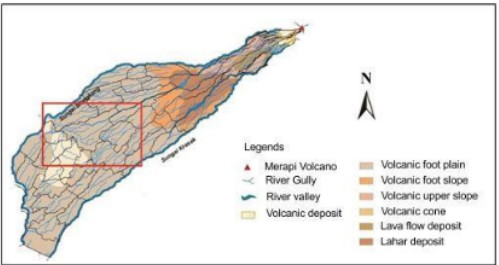
Fig. 2. Geomorphologic map of the southwestern slope of Merapi volcano (Setyawati & Ashari, 2017). Red box shows situation of the research area.
