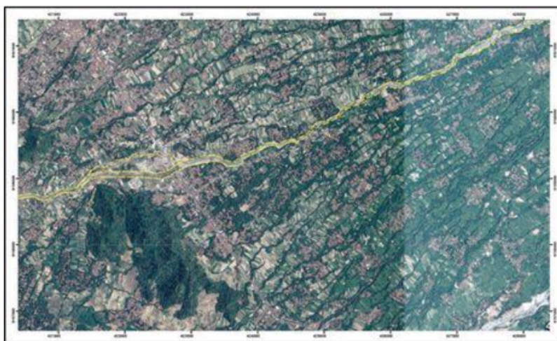
Fig. 14. Modern Kali Putih. Dash line shows the old channel of modern Kali Putih (Source: Google Earth).
