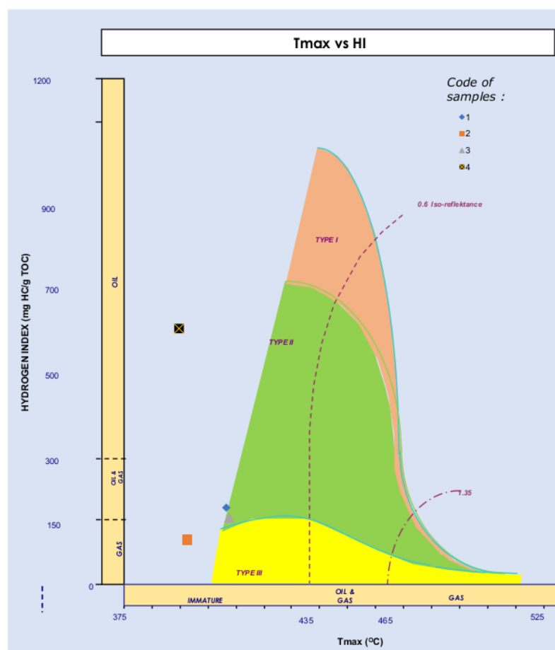
Figure 7. HI vs Tmax graphic.
