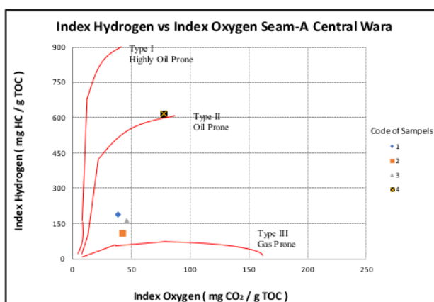
Figure 8. Plot HI vs OI.
