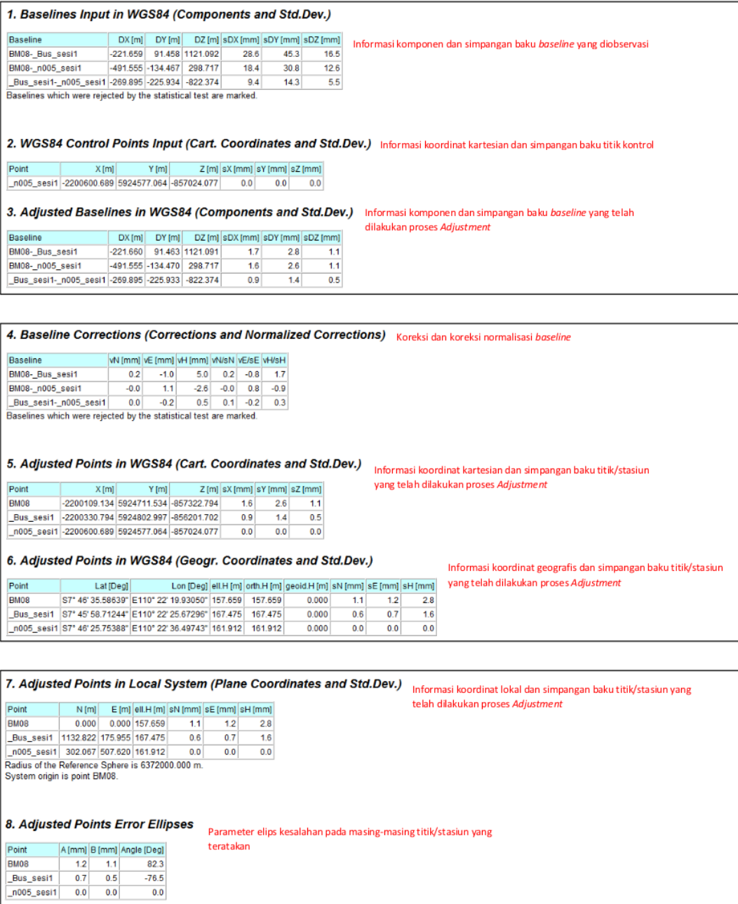
Gambar 30. File report hasil perataan jaring
