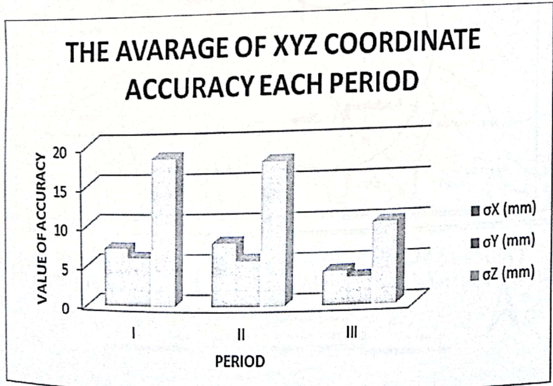
Figure 2. Graph of accuracy of coordinates X, Y and Z each period
