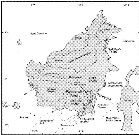
Fig. 1 Simplified physiography of Kalimantan (Witts et al., 2012)
