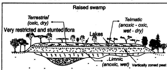
Fig. 8 Peat swamp environment model approaching in research area (modified from McCabe, 1984 in Thomas, 2013).
