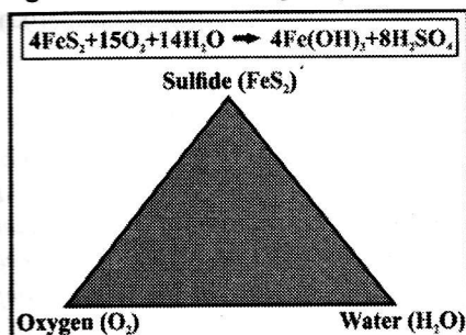
Fig. 10 Formation of acid drainage
