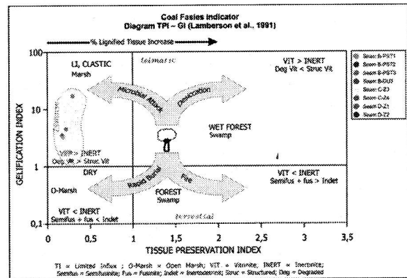
Fig. 6 Coal facies (according to Lamberson et. al, 1991) in Tanjung coal. The coal was deposited in Marsh in limnic state (low moor) and dominated by microbial attack process.
