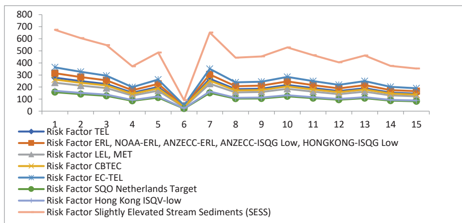
FIGURE 6. Risk Factor Value at fraction 84 \mu\text{m} (150 mesh)
