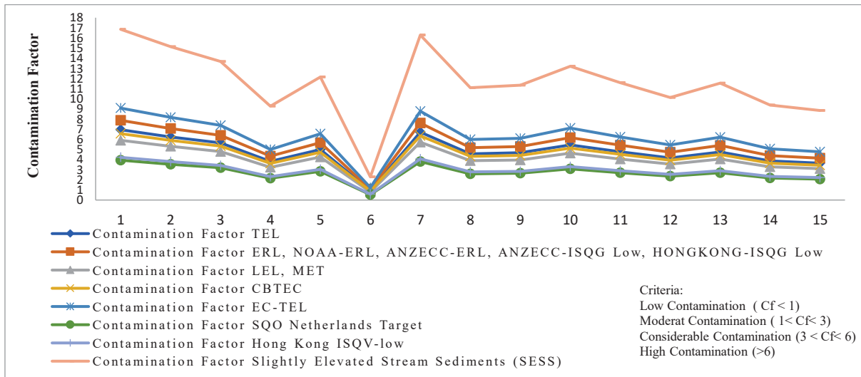
FIGURE 3. Contamination Factor Value at fraction 84 μm (150 mesh)
