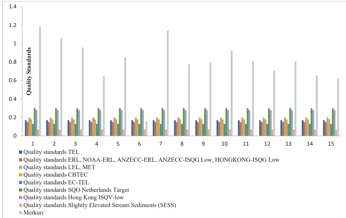
FIGURE 2. Quality standardssediment at a fraction of 84 \mu\text{m} (150 mesh)
