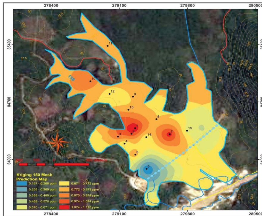
FIGURE 5. Mercury Zoning for Sarantanagan Lake
