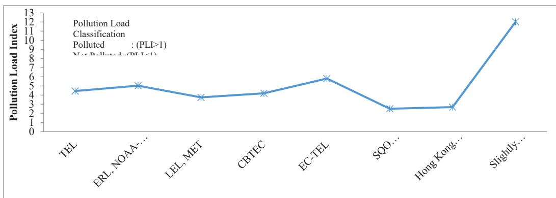
FIGURE 4. Pollution Load Index at a fraction of 84 μm (150 mesh)
