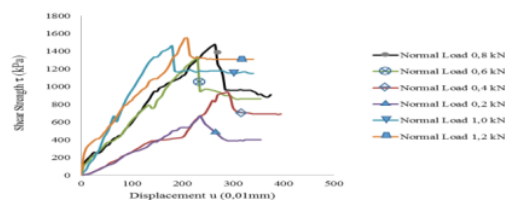
Fig. 3: Shear Strength vs Displacement Peak Condition
