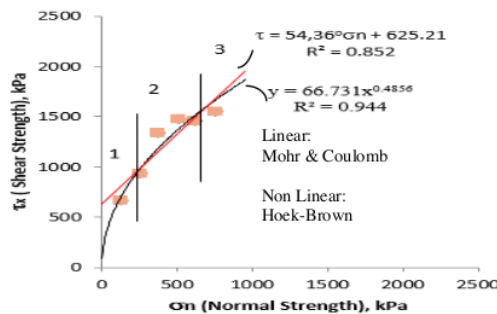
Fig. 6: The Region of Mohr & Coulomb Hoek-Brown results
