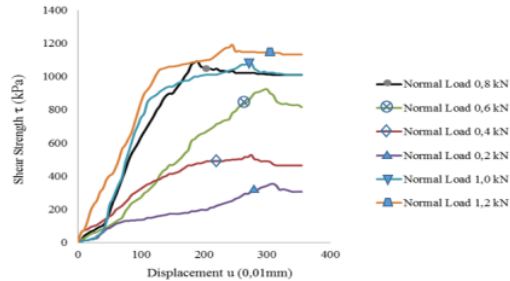
Fig. 4: Shear Strength vs Displacement Residual Condition
