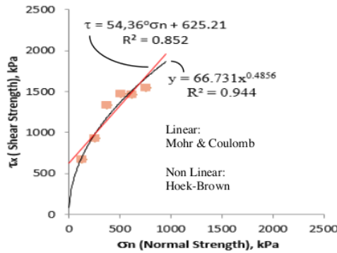
Fig. 5: Comparison of Mohr & Coulomb and Hoek-Brown
