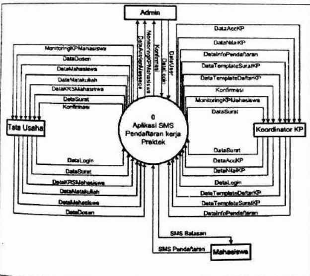
Gambar 2. DFD level 0
