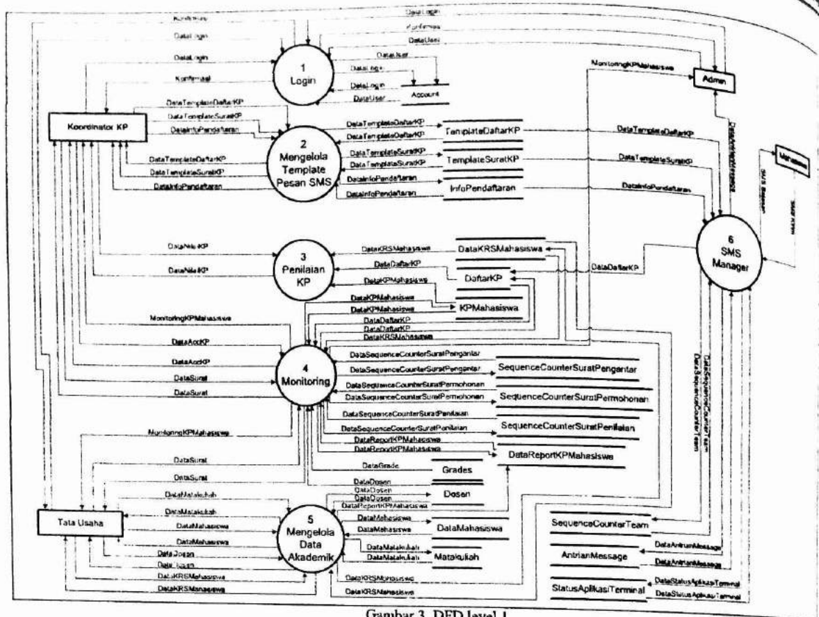
Gambar 3. DFD level 1
