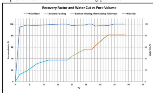
Figure 5. PV Injected vs Recovery Factor for Core Mesh 30
