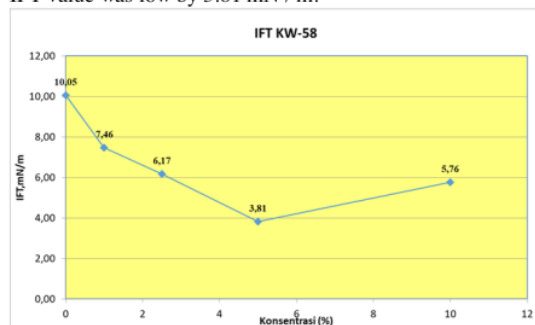
Figure 3. IFT vs U-Champ Concentration Chart Plot.
