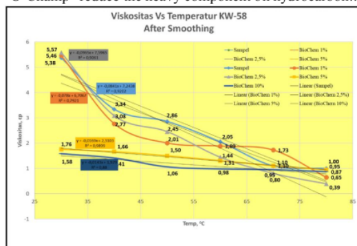
Figure 2. Viscosity vs Temperature Chart Plot
