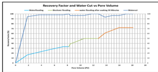
Figure 6. PV Injected vs Recovery Factor for Core Mesh 40
