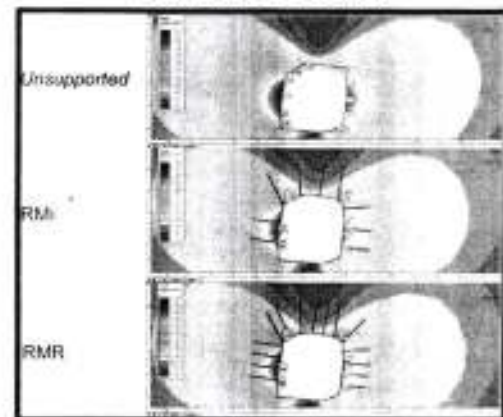
Gambar 4.6 Pemodelan Nilai Total Displacement KN-EXP DRIVE
